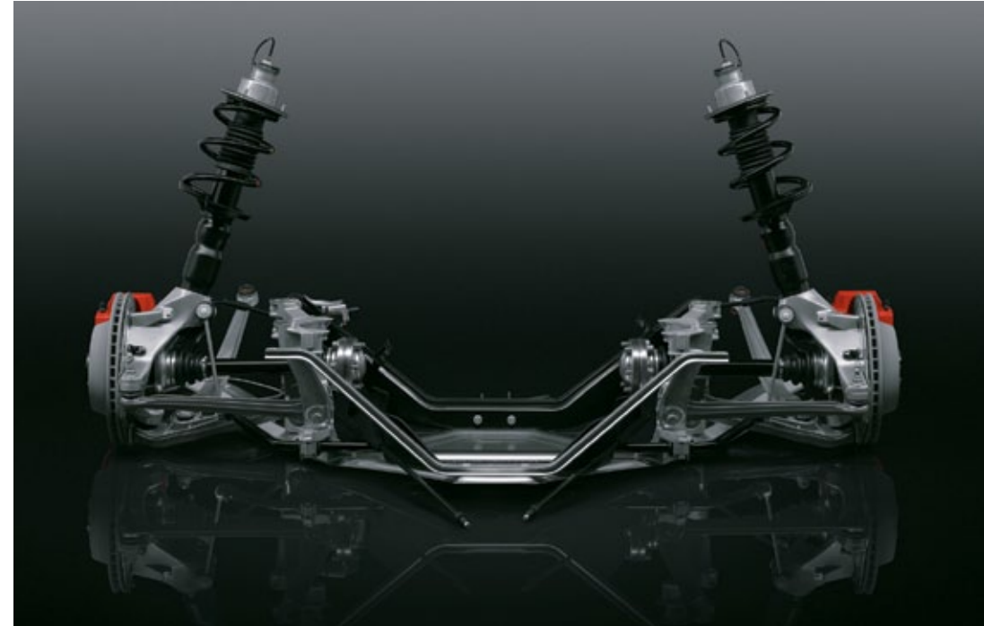
Lightweight spring-strut rear axle on the Cayman S
