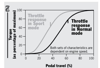
Comparison of the ETC characteristic curve in Normal and Sport modes
